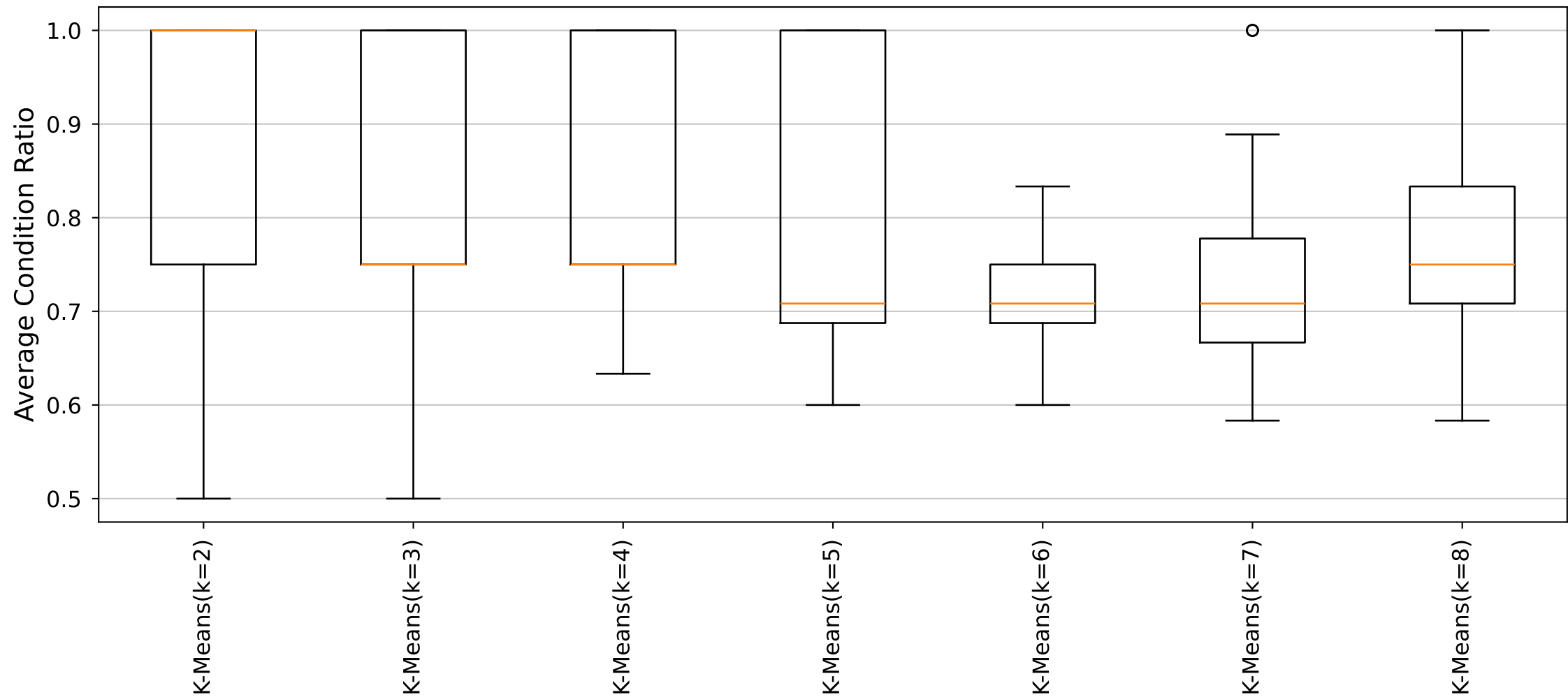
YARA Rules Average Condition Ratio Distribution (Cluster16_Size8 dataset)
